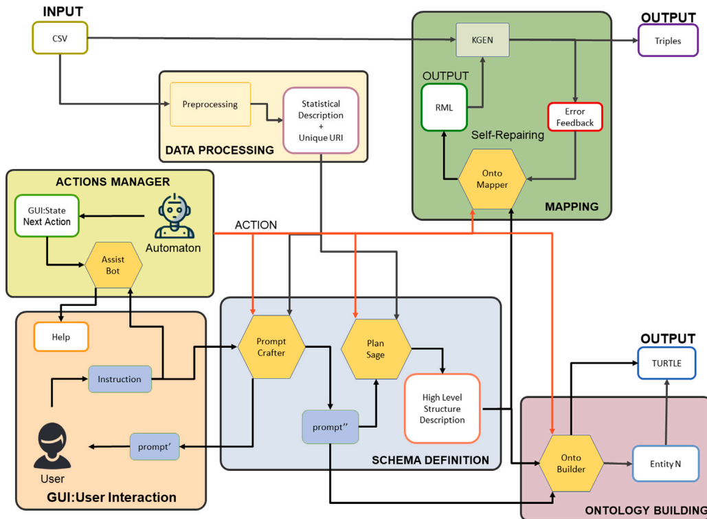
Fig. 1. The Architecture Diagram. This figure illustrates the workflow for enhanced ontology engineering using LLMs. It details the flow from data input, through the various stages of processing, actions management, schema definition, to the final output in ontology format. The system is composed of the following key modules: (A) GUI: User Interaction: This module represents the user's interaction with the system. It includes a help interface and allows the user to input prompts, which are then processed by the Actions Manager. (B) Actions Manager: This module manages the state and actions of the system. It includes the Assist Bot, which assists in determining the next actions based on the GUI state, and interacts closely with the user via the Automaton. (C) Data Processing: This stage involves preprocessing the input data (e.g., CSV files), generating a statistical description, and assigning unique URIs for further processing. (D) Schema Definition: This module includes the Prompt Crafter and Plan Sage, which work together to define the high-level structure of the ontology. The output from this module is a detailed prompt that guides the ontology building process. (E) Ontology Building: This module processes the high-level structure description to generate the ontology and mapping to generate the ontology in the desired formats (e.g., TURTLE and entity N triples). (F) Mapping: This module handles the self-repairing mechanism and error feedback. It includes Onto Mapper, which converts the high-level structure into a mapping format (RML) and generates the RDF data.
